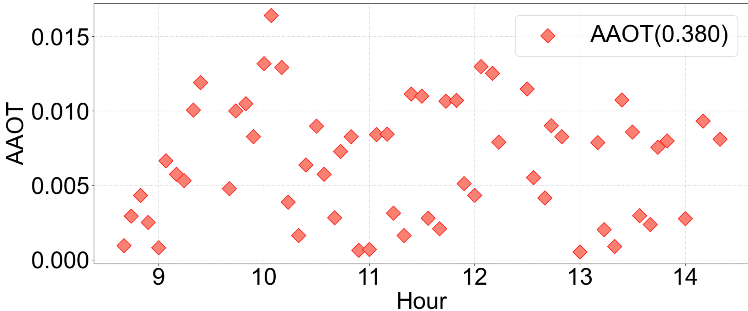
AAOT in Chiba for 2023.11.28
