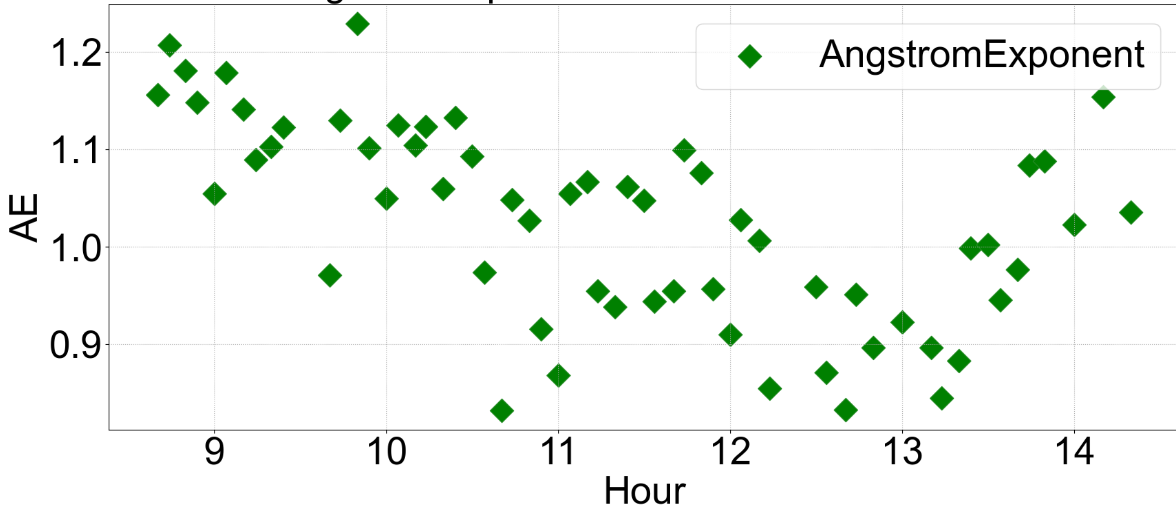
AngstromExponent in Chiba for 2023.11.28
