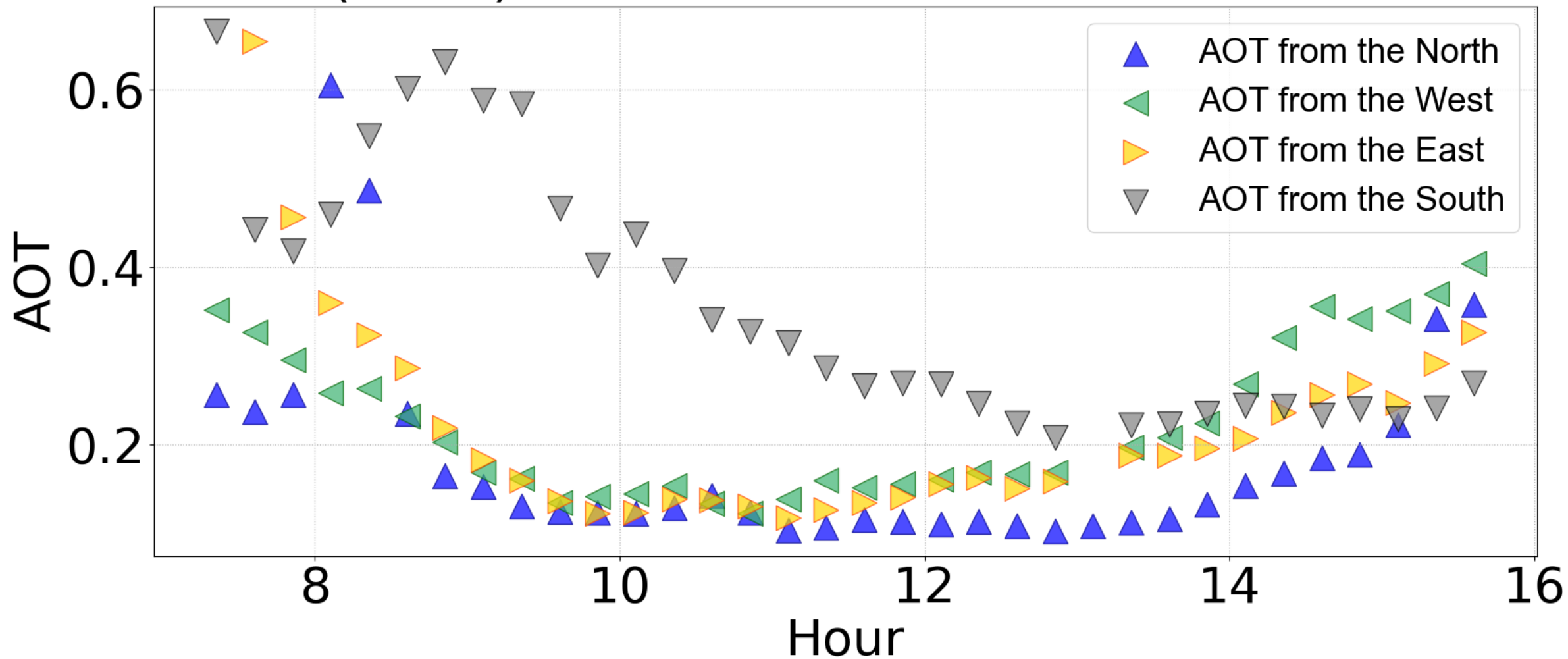
AOT(0.357) of MAX-DOAS in Chiba for 2023.11.28
