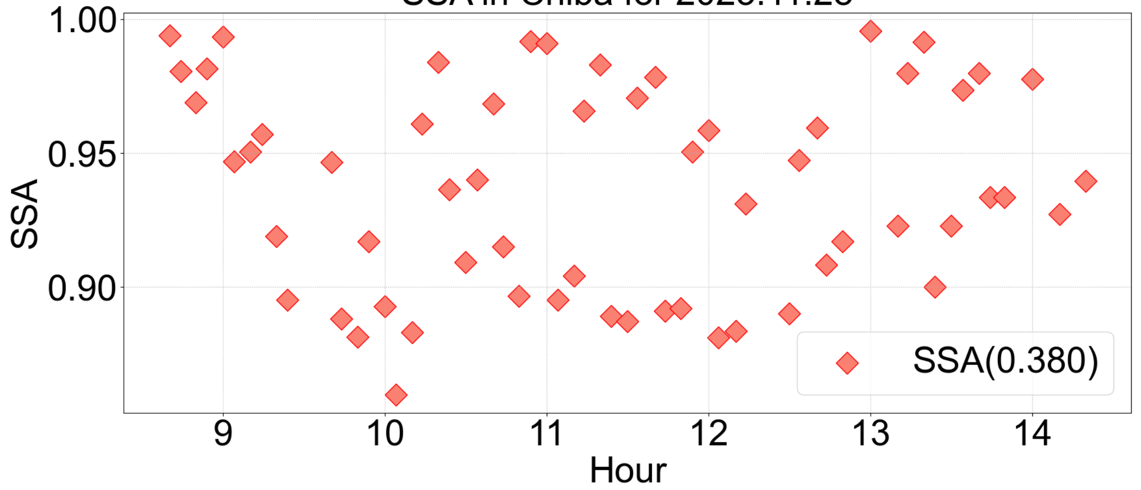
SSA in Chiba for 2023.11.28
